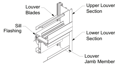
Fig. 3.2 Multi-Section High
