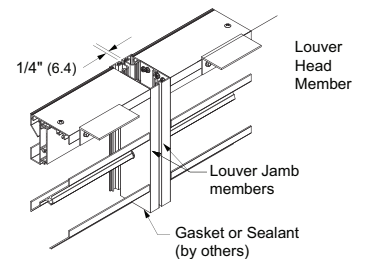
Fig. 3.4 Visible Mullion Interior
