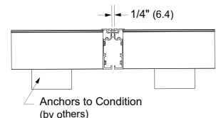
Fig. 3.5 Visible Mullion
