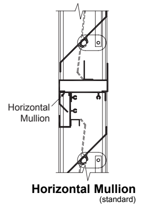
Vertical Section †Screen adds approximately 3/16" (5) to louver depth.
