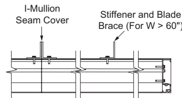
Hidden Vertical Mullion
