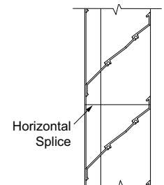
Horizontal Mullion
