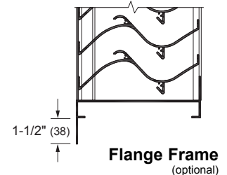
Hidden Vertical Mullion (optional)
