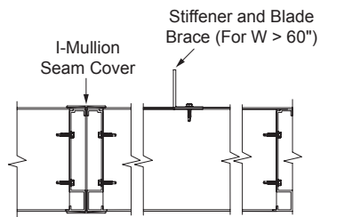
Hidden Vertical Mullion (optional)
