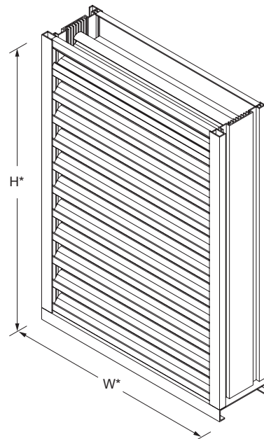
Model ECD-545-MD (standard) *Louver dimensions furnished approximately 1/2" (13) undersize.
